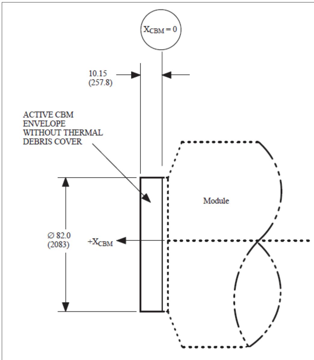
Figure 10: Typical ACBM Static Envelope as mounted on a Pressurized Element Axial Port
