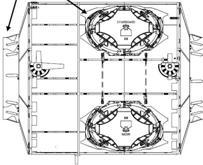
Figure 8: Typical installed locations of the CBM.
