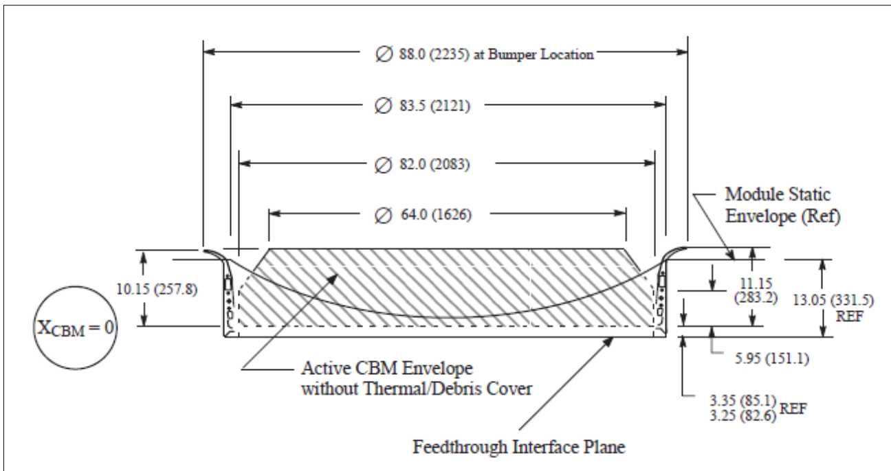
Figure 11: Typical ACBM Static Envelope when installed on a Pressurized Element Radial Port
