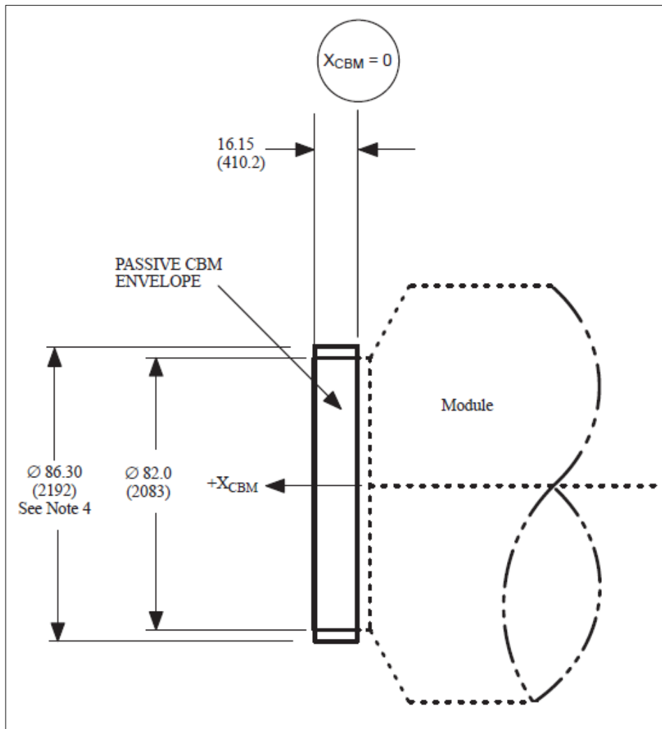
Figure 9: PCBM Static Envelope as mounted on a Pressurized Element Axial Port
